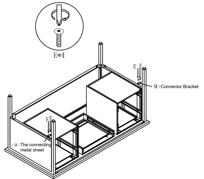
Diagram A(Double Pedestal Desk)
