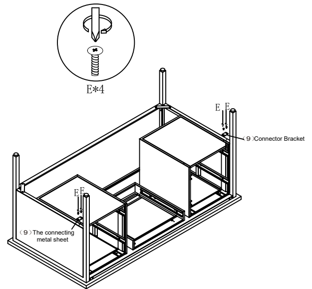
Diagram A(Double Pedestal Desk)
