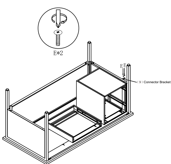
Diagram B(Single Pedestal Desk)
